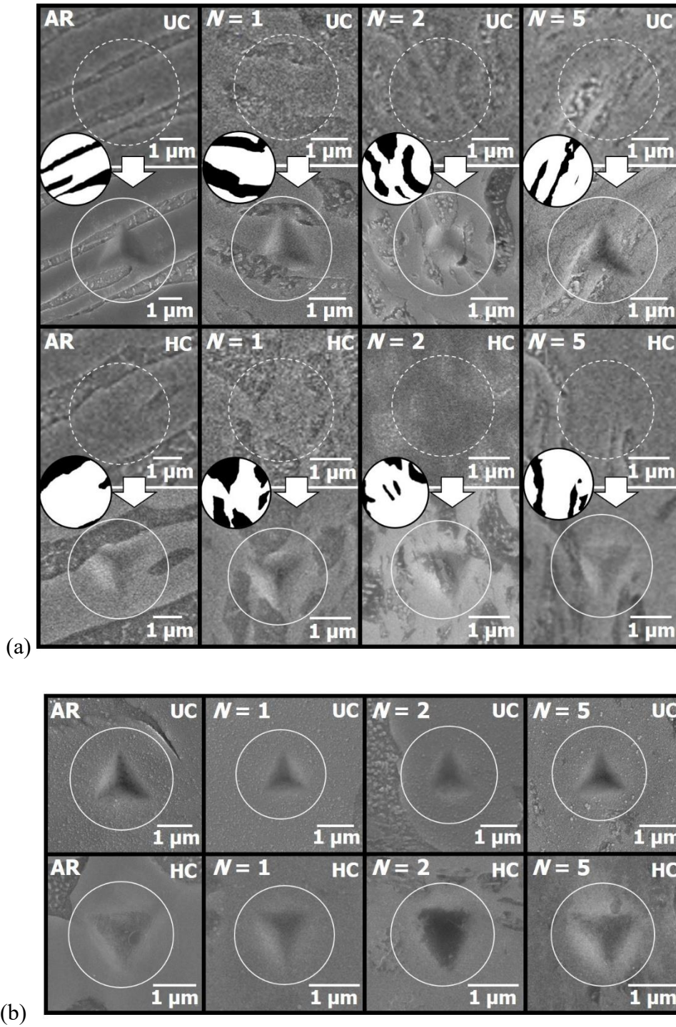
Figure S2 SEM images of uncharged (UC) and hydrogen-charged (HC) samples (a) before and after the indentation of P_{\max} = 10 mN and (b) after the indentation of P_{\max} = 5 mN only in the FCC phase.
