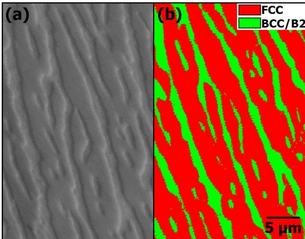
Figure S1 Representative EBSD results of AR sample; (a) SEM image and (b) phase map.
